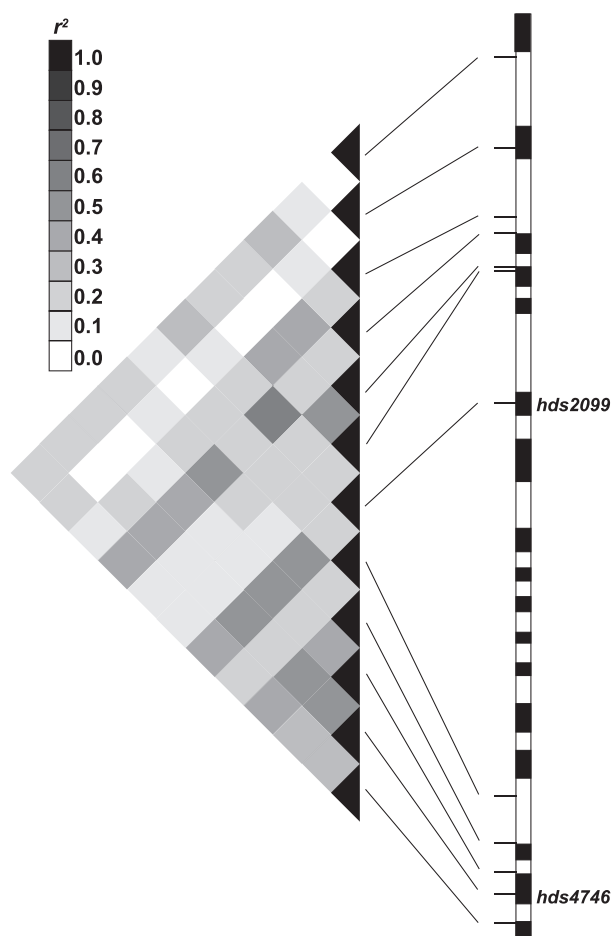
Fig. 4 Exon/intron structure and linkage of single nucleotide polymorphisms (SNPs) within the Eucalyptus globulus hds locus. Illustrated are 12 SNPs genotyped in this locus. Linkage across (E)-4-hydroxy-3-methylbut-2-enyl-diphosphate synthase ( hds ) is shown as well as the locations of exons (closed bars) and introns (open bars). The locations of the two nonsynonymous SNPs are shown in exons 6 and 16.
