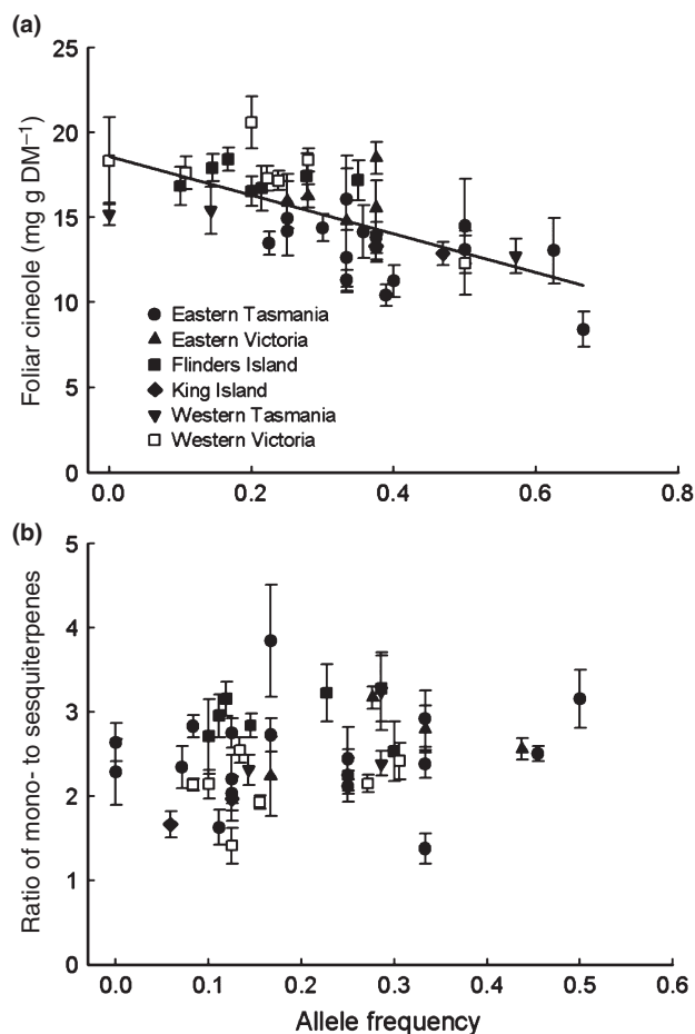
Fig. 5 Relationship between variation in foliar 1,8-cineole concentration and the allele frequency for hds2099 . (a) Cineole content (average per Eucalyptus globulus population) vs the allele frequency of the minor allele of hds2099 (average within each population); (b) ratio of mono- to sesquiterpenes vs the minor allele frequency of ggpps103 . DM, dry matter.
